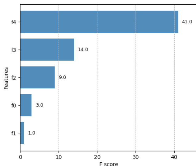
Figure 10. Importance of features in the XGBoost model
