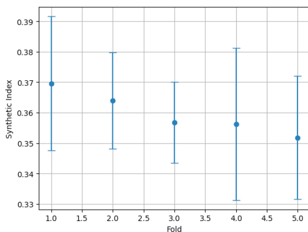
Figure 2. SMPI average and standard deviation (cross-validation)
