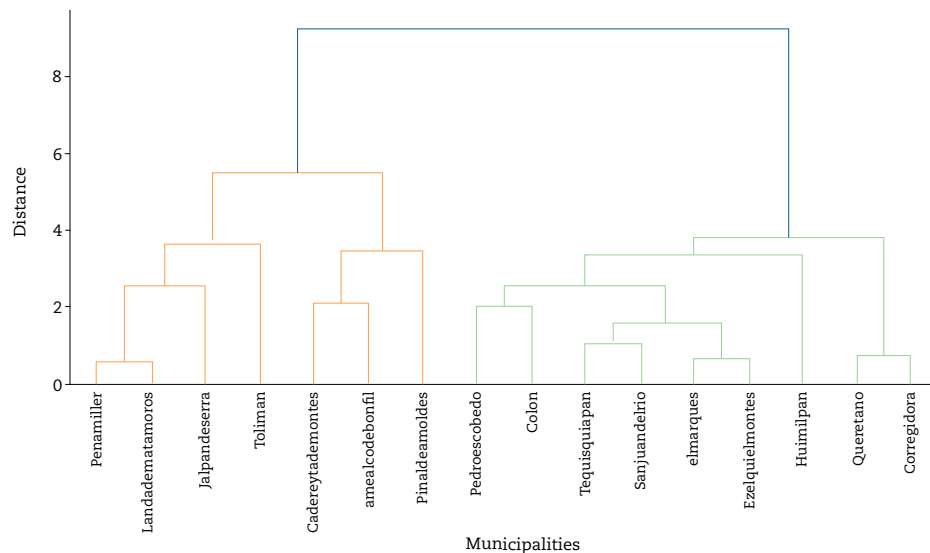
Figure 9. Dendrogram of hierarchical clustering for municipalities in Querétaro
