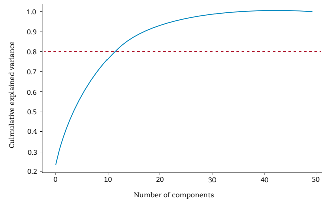
Figure 1. Elbow plot for component retention
